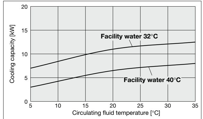
HRL200-W□-20 (CH1)
