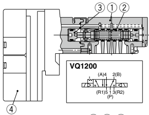
VQ1100 (A)4 2(B) (R)1 5 3 (R)2 (P)
