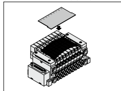
Name plate [-N] VVQ1000- N C -Station (1 to Max. stations) (-X4)
