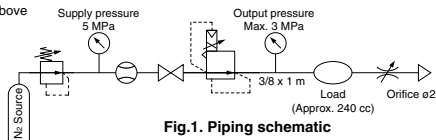
Fig. 1. Piping schematic
