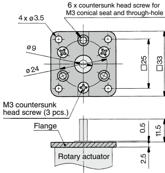
Flange assembly for C□RB2F□□10 Part no.: P211070-2
