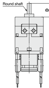
Double shaft/CDRB2□JU
